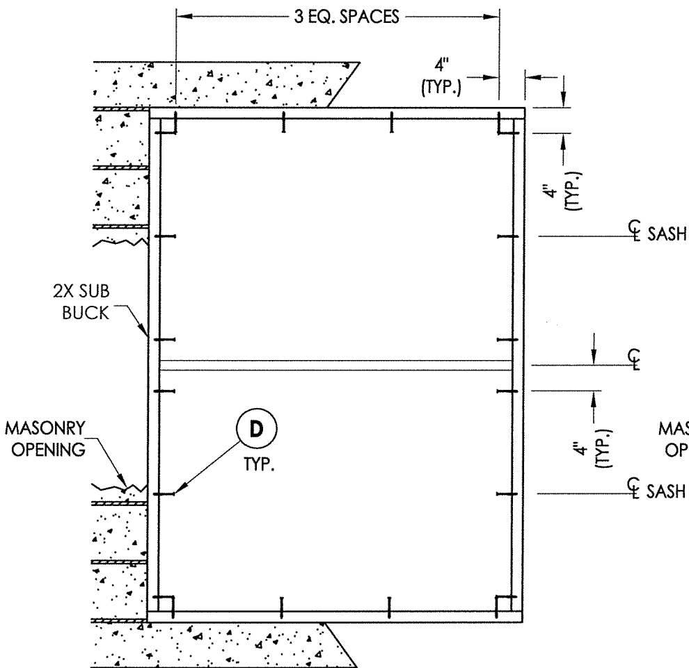
BUCK ANCHORING
